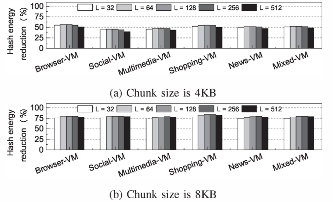
Fig. 6: Percentage of reduced energy using energy-aware hashing of FLIC with different sample lengths and chunk sizes, compared to full hashing.
